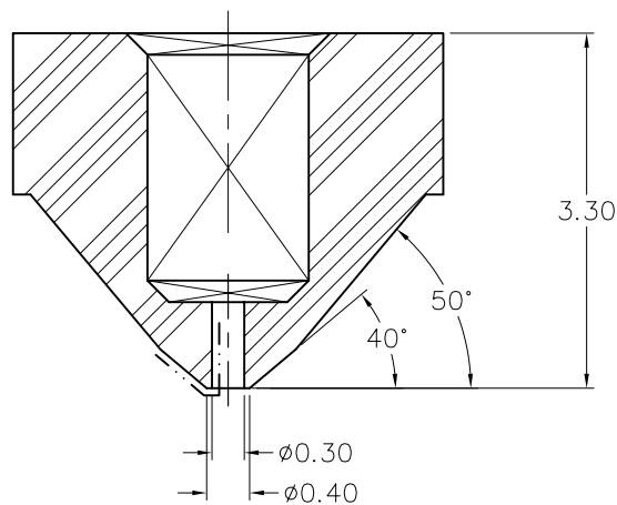
SECTION X-X
